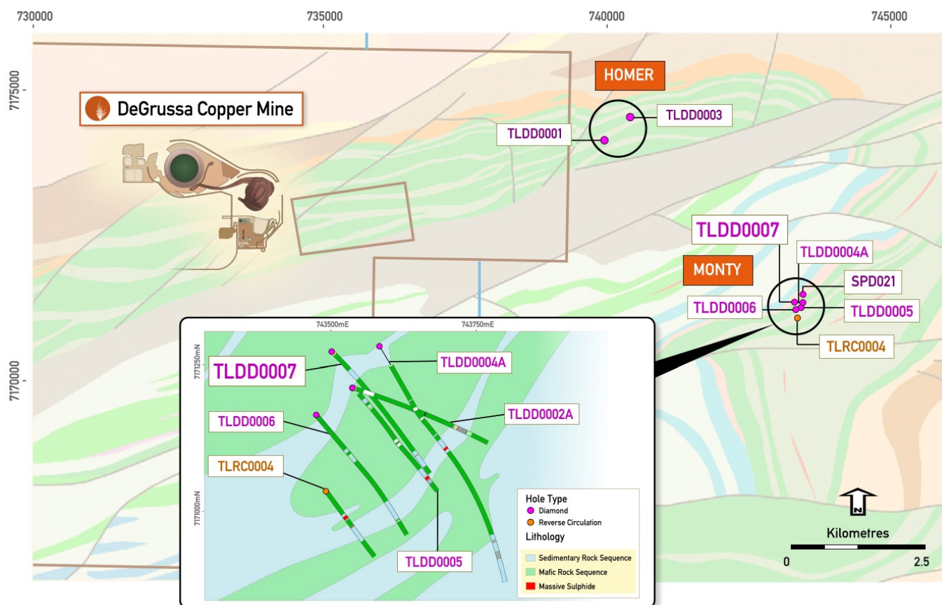
Figure 2 – Location of recent drilling relative to the DeGrussa Copper Mine
